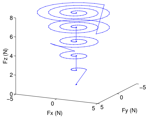
Figure 11: 3-D force trajectory based on Archimedean spiral.
