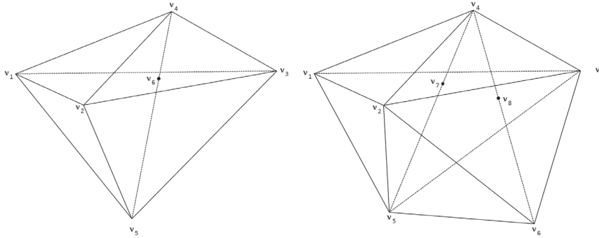
FIG. 2.2. Diagram denoting the strategy used to deal with obtuse tetrahedra. We split the obtuse angle \omega_4 to create three virtual tetrahedra used within the local solver.
