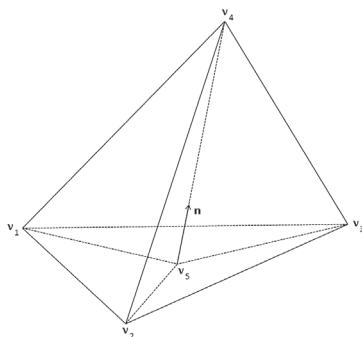
FIG. 2.1. Diagram denoting components of the local solver. We compute the value of the approximation at the vertex v_4 from the values at vertices v_1 , v_2 and v_3 . The vector \mathbf{n} denotes the wave propagation direction that intersects with the triangle \Delta_{1,2,3} at v_5 .
