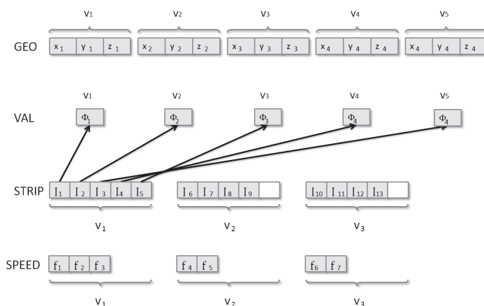
FIG. 3.2. One-ring-strip data structure: in this figure, T_i is a tetrahedron, x_i , y_i and z_i represent the coordinates of the i th vertex, f_i is the inverse of speed on a vertex. \Phi_i denotes the value of the solution at the i th vertex. I_i in STRIP represents the data structure for the one-ring strip of the i th vertex each of which has q indices pointing (shown as arrows) to the value array.
