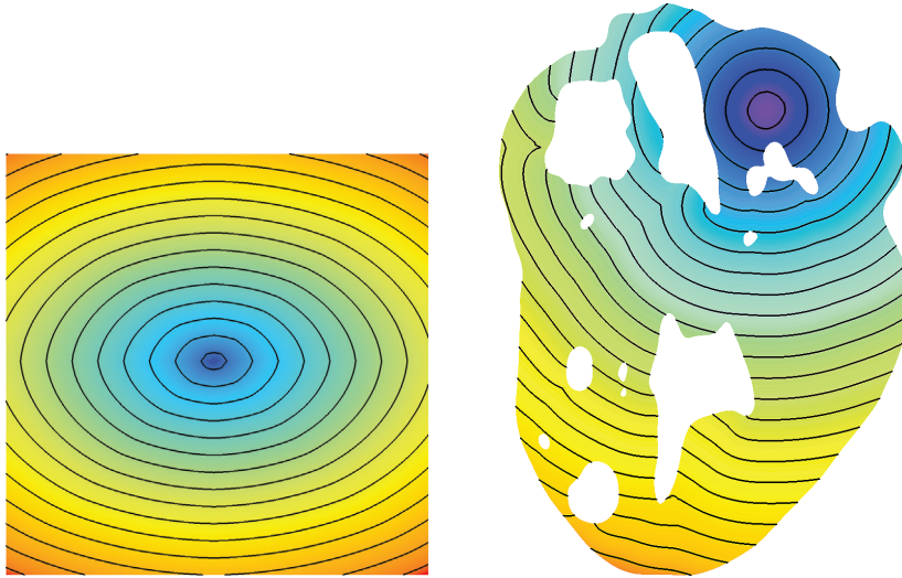
FIG. 4.2. Color maps and level curves of the solutions on the cube and heart meshes. Left: the elliptic speed function (Speed 2). Right: the isotropic constant function (Speed 1).
