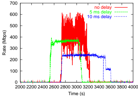
Figure 2: Synchronous replication: FCIP throughput for different delay values
