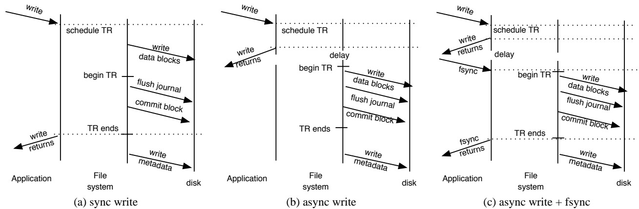
Figure 4: Event sequence for a synchronous write, an asynchronous write, and asynchronous write followed by a fsync.
