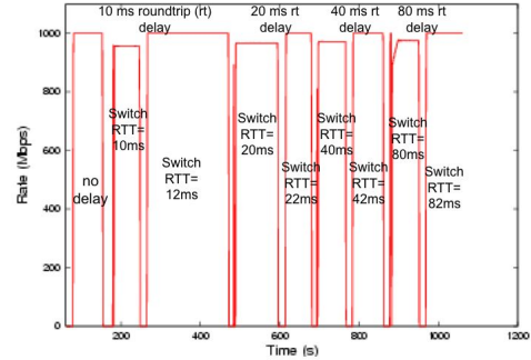
Figure 3: Asynchronous replication: FCIP throughput with different delay values and FCIP switch parameters settings.
