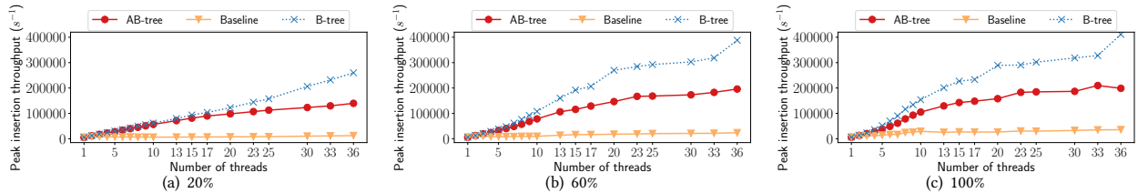
Figure 12: Insertion throughput vs number of threads with large buffer
