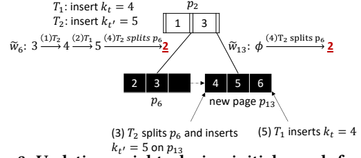
Figure 3: Updating weights during initial search for insertion point may lead to undercount due to concurrent splits. \phi denotes an uninitialized weight.
