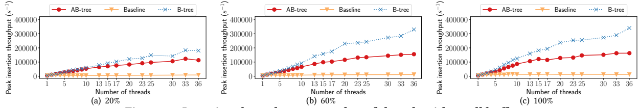
Figure 11: Insertion throughput vs number of threads with small buffer
