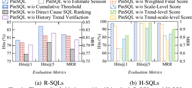
Fig. 6. The result of ablation on identifying both R-QLS and H-QLS.
